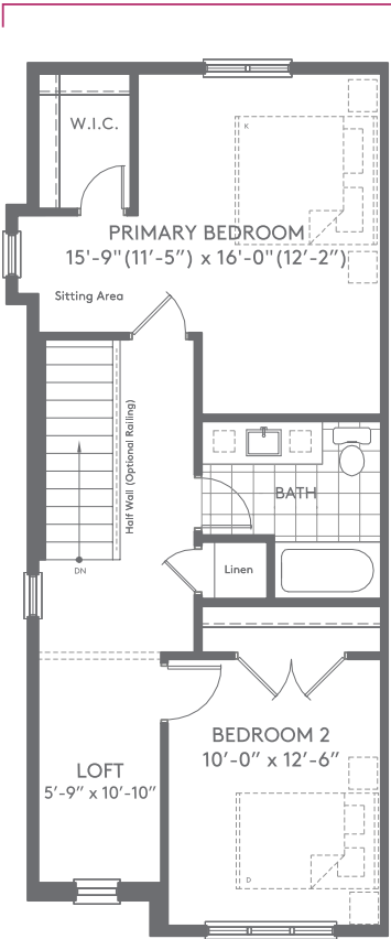
SECOND LEVEL
