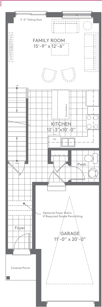
MAIN LEVEL
