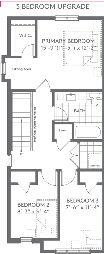
SECOND LEVEL
