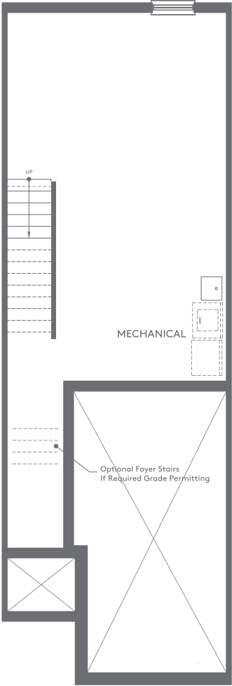
BASEMENT LEVEL
