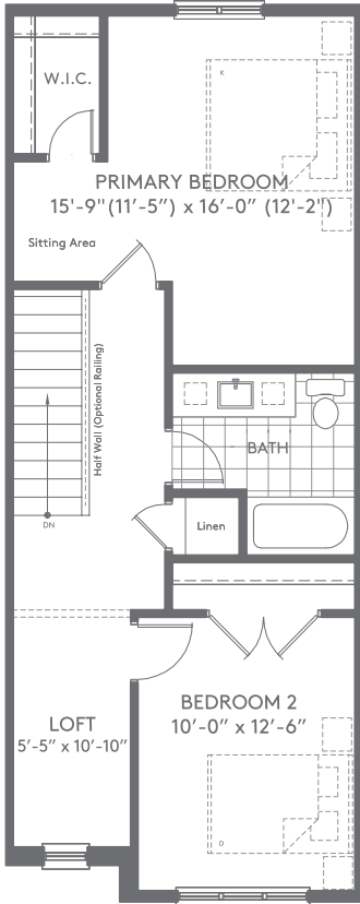
SECOND LEVEL
